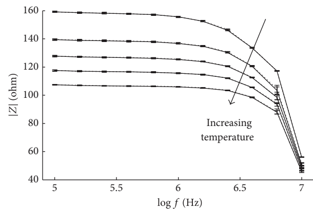
FIGURE 5: Impedance modulus spectrum for the samples at 78 mg/dL, in static (dotted curve) and dynamic (solid curve) conditions at room temperature and at 32, 37, 42, and 47^\circ\text{C} (from top to bottom). Data reported are mean \pm SE.
