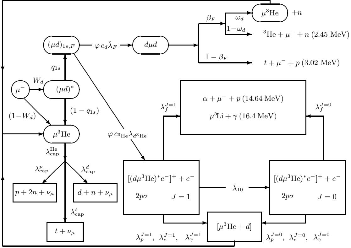
Fig. 1. Scheme of \mu -atomic and \mu -molecular processes when a negative muon is stopped in a D_2 + {}^3\text{He} mixture.
