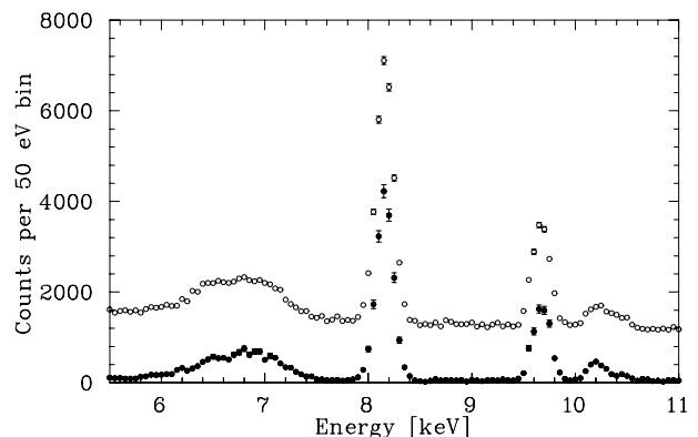
Fig. 3. Energy spectra of events detected by the \text{Ge}_S detector in run I with (full circles) and without (open circles) the del- e criterion.
