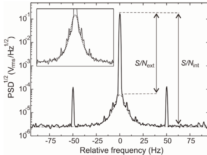
Fig. 2. Square root of the power spectral density (PSD) of the magnetometer output frequency relative to the Larmor frequency of \nu_L = 7032 \text{ Hz} (averaged 20 times). The spectrum was measured with a 1 Hz resolution bandwidth. The signal-to-noise ratio S/N_{\text{int}} is approximately 66 000. The sidebands are due to imperfectly shielded magnetic field components oscillating at the 50 Hz power-line frequency. The dotted line is an approximation of the pedestal. The signal-to-noise ratio S/N_{\text{ext}} due to external field noise is found to be approximately 2600.
