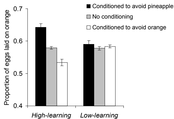
Figure 2: Response of oviposition substrate preference to conditioning, measured for crosses between replicate lines within selection regimes; bars represent \pm one standard error. Significant interaction between the selection regime and the conditioning treatment ( F_{2,6} = 30.9, p < 0.001 ) indicates differences in learning ability between the two sets of crosses: crosses between the experimental lines responded to conditioning ( F_{2,6} = 30.7, p < 0.001 ), whereas crosses between the control lines did not ( F_{2,6} = 0.9, p = 0.43 ).
