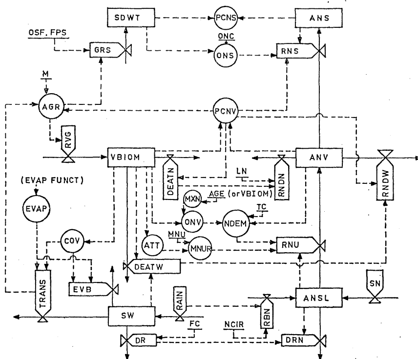
Fig. 2. Main structural features of plant nitrogen model. \rightarrow flow of material; \cdots\rightarrow flow of information; \square state variable; \square rate of change; \circ auxiliary variable; - parameter. SDWT seed weight; PCNS N-conc. in seed; ANS amount of N in seed; OSF onset of seed-fill; FPS fraction of photosynthate to seeds; GRS growth rate of seeds; ONC optimum N-conc in seeds; ONS optimal amount of N in seeds; RNS rate of nitrogen translocation to seeds; M proportionality (or transpiration) factor; AGR actual total growth rate; RVG rate of vegetative growth; PCNV N-conc. in vegetative biomass; VBIOM vegetative biomass; DEATN death rate of VBIOM due to N-deficiency; LN limiting (residual) N-conc; RN rate of N loss to dead plant material due to N-deficiency; ANV amount of N in live biomass; RNDW rate of N-loss to dead plant material due to water deficiency; EVAP potential evaporation; COV plant cover; DEATW death rate of VBIOM due to water deficiency; ATT available transfer tissue; MNU maximum N-uptake rate per unit of transfer tissue; MNUR maximum actual N-uptake rate; MXN maximum N-concentration in VBIOM ; ONV maximum N-content of VBIOM ; NDEM N-demand; TC time constant ( \text{TAU}_2 ); RNU rate of N-uptake; TRANS transpiration; EVB - evaporation from bare soil; SW soil water content; DR - rate of drainage; RAIN precipitation; FC field capacity; NCIR N-conc in rainfall; RBN rain borne N; ANSL amount of N in soil; DRN loss of N in drainage; SN seedling N
