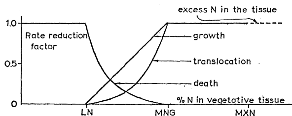
Fig. 1. A schematic representation of the effect of nitrogen concentration in the plant on net growth rate, death rate and the rate of nitrogen translocation to the seeds ( LN low, residual N-conc. in plant; MNG minimum N-conc. needed for unrestricted growth)
