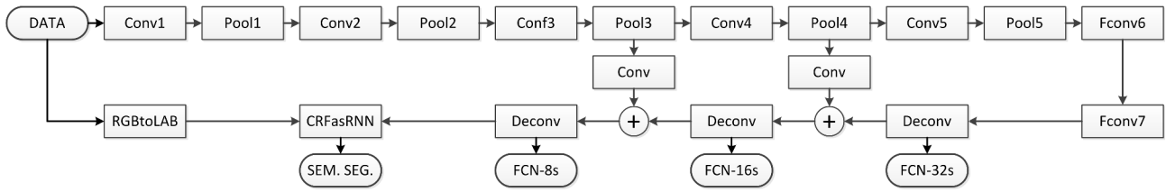
Figure 2. Schematic overview of the Neural Network: The network consists of (fully) convolutional, pooling and deconvolutional layers. Further, the option of early exit exists, which results in coarse semantic segmentations (FCN-XXs). The pixel accurate segmentation (SEM. SEG.) is attained by adding an RGB to LAB color space conversion (RGBtoLAB) and a conditional random field represented as recurrent neural network (CRFasRNN).
