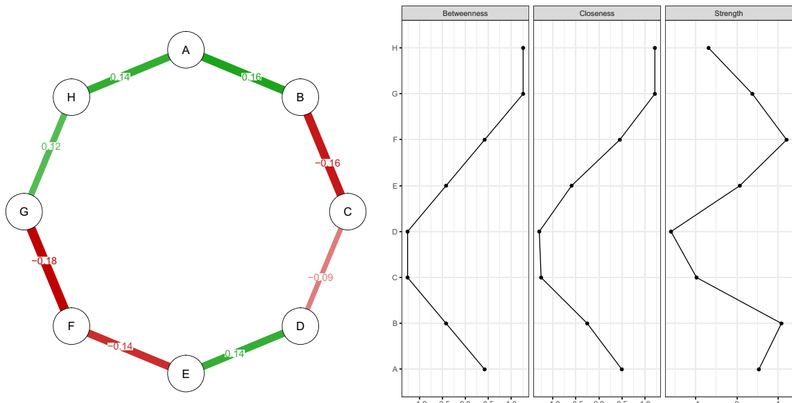
Fig. 2 Estimated network structure based on a sample of 500 people simulated using the true model shown in Fig. 1 (left panel) and computed centrality indices (right panel). Centrality indices are shown
