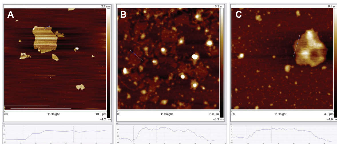
Figure 3 AFM height images of (A) GO sheets, (B) GO and SGI complex, and (C) GO and ssDNA complex on mica substrates.
