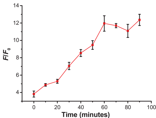
Figure 5 Effects of reaction time of SYBR Green I SGI on F/F_0 in the absence and presence of 1.2 \mu M Hg^{2+} in the test conditions of 8 \mu L SGI, 80 nM MC, and 2 \mu g/mL graphene oxide.
