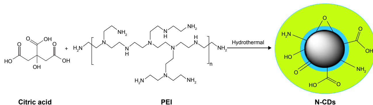
Figure 1 Schematic illustration of hydrothermal synthesis of N-CDs using citric acid and PEI. Abbreviations: N-CDs, nitrogen-doped carbon dots; PEI, polyethylenimine.
