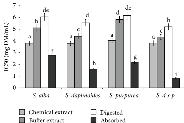
FIGURE 4: Effect of extraction system on reducing power of phytochemicals from bark of different Salix genotype. Bars (means) followed by the different letters differ significantly (Tukey-test, P < 0.05 ).
