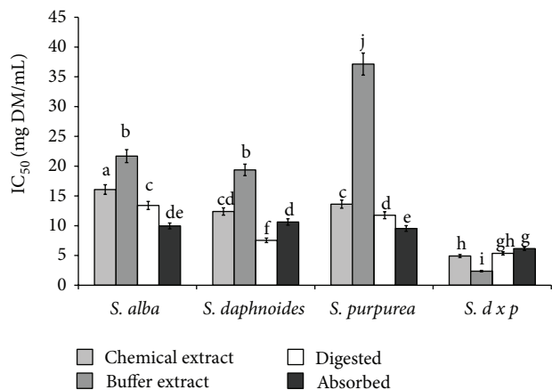
FIGURE 2: Effect of extraction system on antiradical activity of phytochemicals from bark of different Salix genotype. Bars (means) followed by the different letters differ significantly (Tukey-test, P < 0.05 ).
