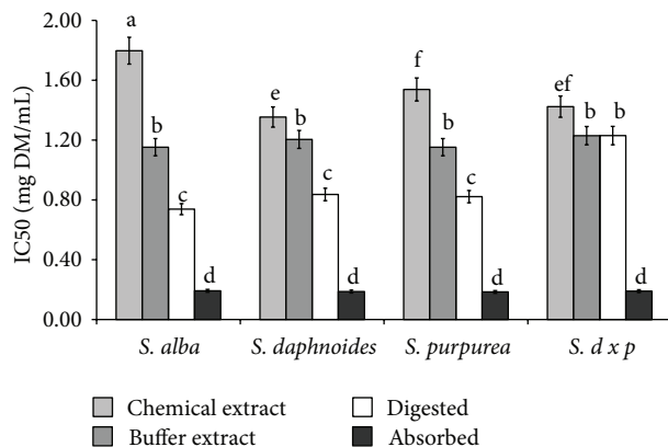
FIGURE 3: Effect of extraction system on chelating power of phytochemicals from bark of different Salix genotype. Bars (means) followed by the different letters differ significantly (Tukey-test, P < 0.05 ).
