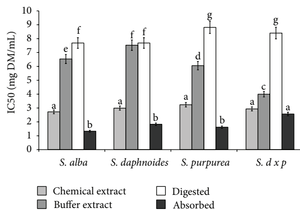
FIGURE 6: Effect of extraction system on XO-inhibitory activity of phytochemicals from bark of different Salix genotype. Bars (means) followed by the different letters differ significantly (Tukey-test, P < 0.05 ).
