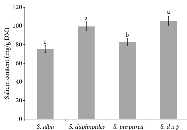
FIGURE 1: Comparison of phenolic glycosides content in Salix bark. Bars (means) followed by the different letters differ significantly (Tukey-test, P < 0.05 ).
