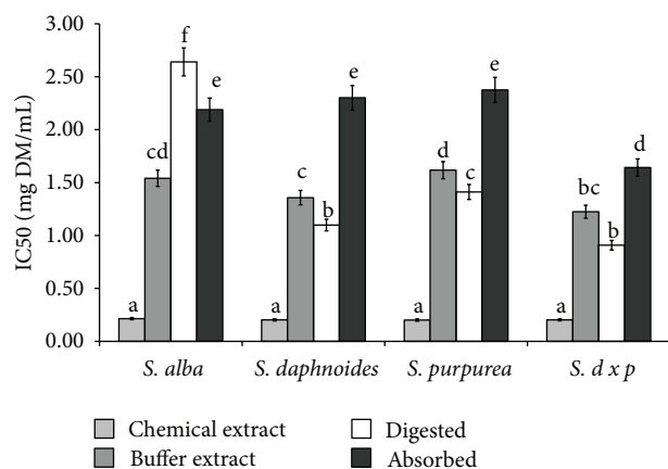
FIGURE 5: Effect of extraction system on LOX-inhibitory activity of phytochemicals from bark of different Salix genotype. Bars (means) followed by the different letters differ significantly (Tukey-test, P < 0.05 ).
