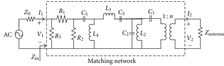
FIGURE 5: Optimized matching network.
