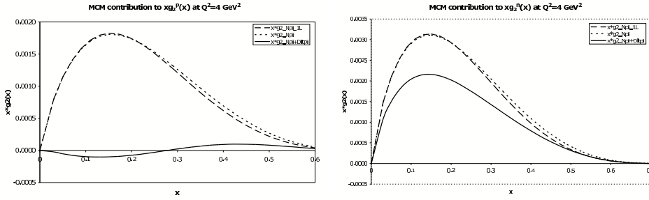
FIGURE 2. Meson cloud Model contributions to g_2 of the proton and neutron. The dashed line is the contribution from longitudinally projected nucleon fluctuations, the dotted line is the total contribution from nucleon fluctuations and the solid line is the total from nucleon and \Delta fluctuations.
