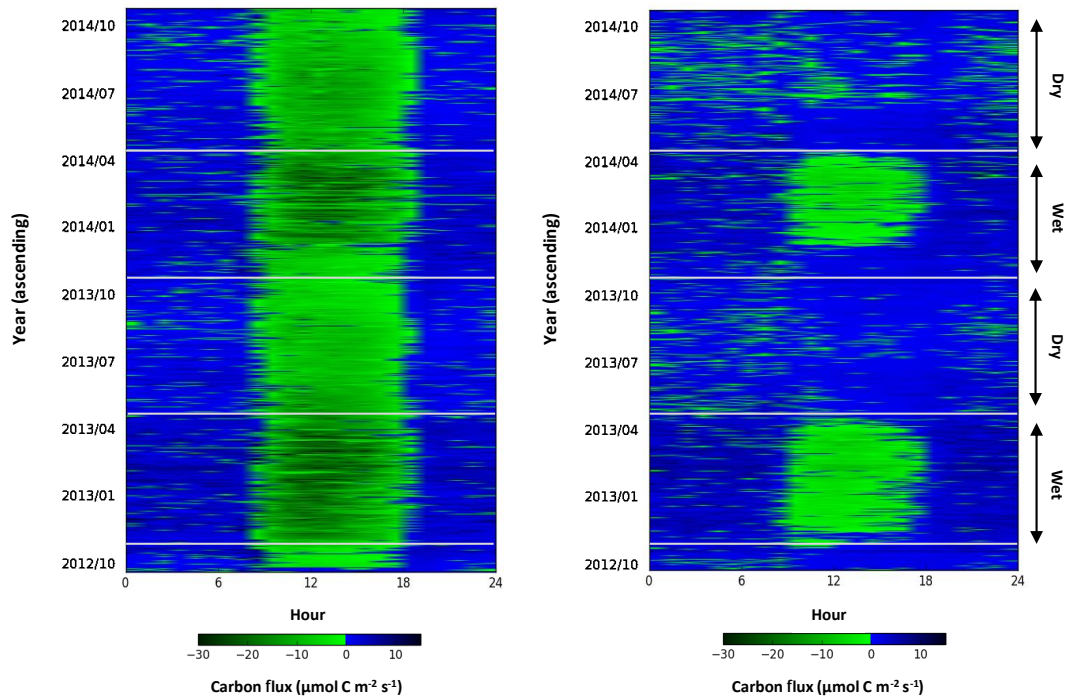
Figure 6. Diurnal ( x axis) fingerprint plot of NEE from the savanna (a) ecosystem (23 m tower) and (b) understory (5 m tower). Measurements shown are for “wet” and “dry” seasons from September 2012 to October 2014 ( y axis) at the Howard Springs OzFlux site, Northern Territory, Australia. Negative NEE represents the uptake of carbon by the savanna, whereas positive NEE represents the loss of carbon from the savanna.
