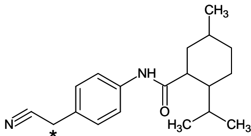
Figure C.1. The structure of [ 14 C]- N-p -benzenenitrile-menthanecarboxamide [FL-no: 16.117], with location of the [ 14 C] label (*).
