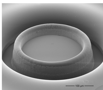
Fig. 3: SEM image of a single microcontainer in poly(lactide acid) (PLLA) after hot embossing. Outer diameter of 300 \mu m, inner diameter of 240 \mu m, and height of 100 \mu m.
