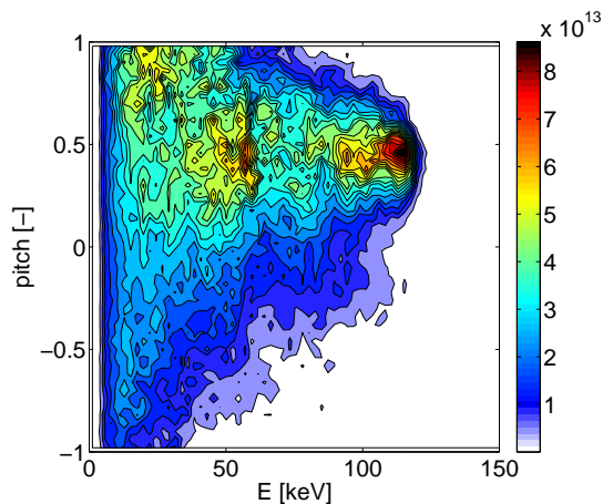
FIG. 5. Central fast-ion distribution function in units of [fast ions pr keV] calculated using TRANSP/NUBEAM.
