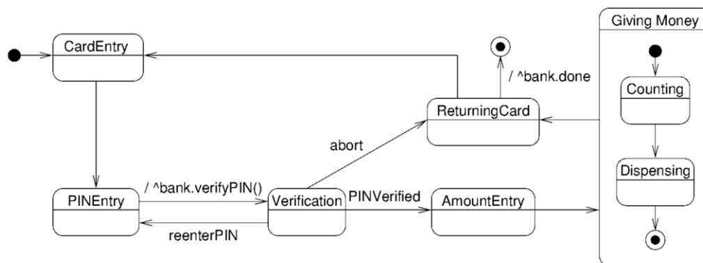
Figure 4 ATM state machine
