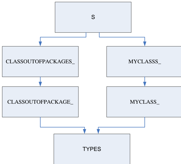
Figure 2 RSL output dependency diagram
