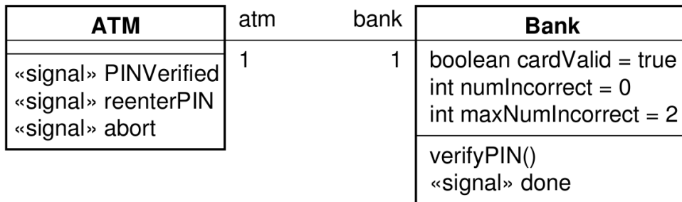
Figure 3 ATM - Bank class diagram
