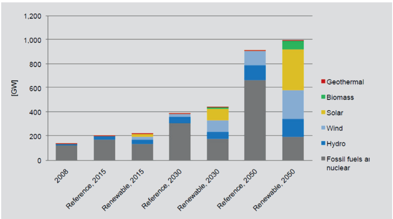
Figure 3. Installed electricity generation capacity by fuel in the reference and renewable scenarios, 2008 to 2050.
