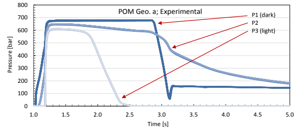
FIGURE 3. Experimental pressures from the pressure sensors in the mold. Sensors positions: P1 = before the gate, P2 = in the part, P3 = in an overflow at the end of the part. Average experimental standard deviation of pressure curves = 1.2 bar.
