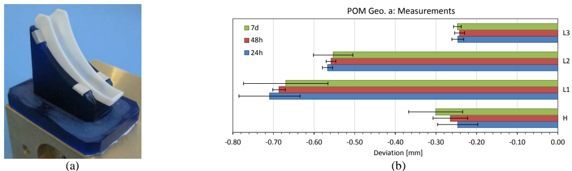
FIGURE 4. (a) Part mounted in the fixture ready for warpage measurements. (b) Average of measurement results on 10 different parts at 24h, 48h, and 7 days after production. Errors bars indicate experimental standard deviation.
