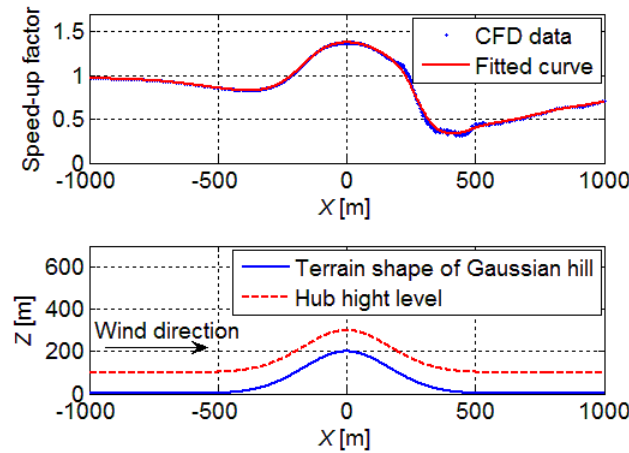
Figure 1: Speed-up factors at the hub height level and shape of the hill
