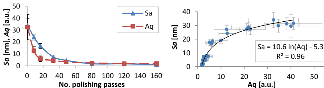
Figure 5; Trend in Sa and Aq surface roughness parameters during 160 polishing passes (left) and correlation of Sa and Aq from all measurements on 5 work pieces (right), with error bars representing \pm one measurement standard deviation.
