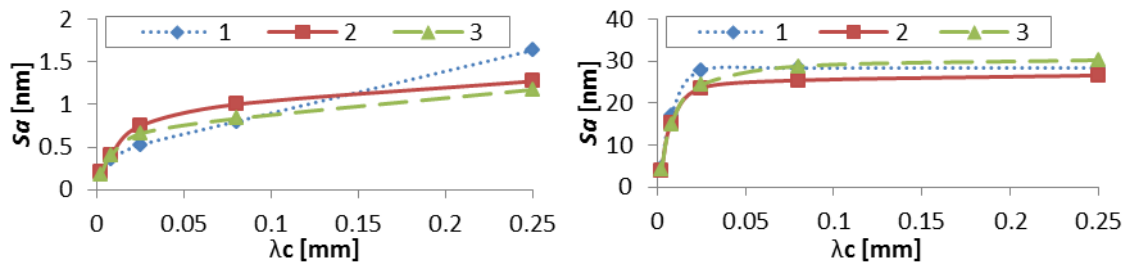
Figure 4; Sensitivity analysis – effect of cut-off length \lambda_c on surface roughness Sa on 3 fine surfaces after 160 polishing passes (left) and 3 rough pre-polished surfaces (right); \lambda_c = 0.25 ; 0.08; 0.025; 0.008 and 0.0025 mm.
