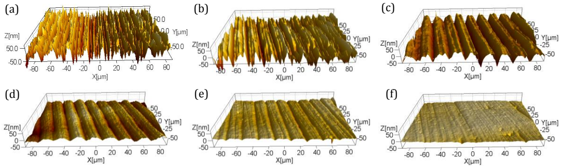
Figure 6; Surface topography after: pre-polishing – 31 nm Sa (a), 8 passes -23 nm Sa (b), 16 passes – 20 nm Sa (c), 32 passes – 8 nm Sa (d), 48 passes – 6 nm Sa (e), and 80 passes – 3 nm Sa (f).
