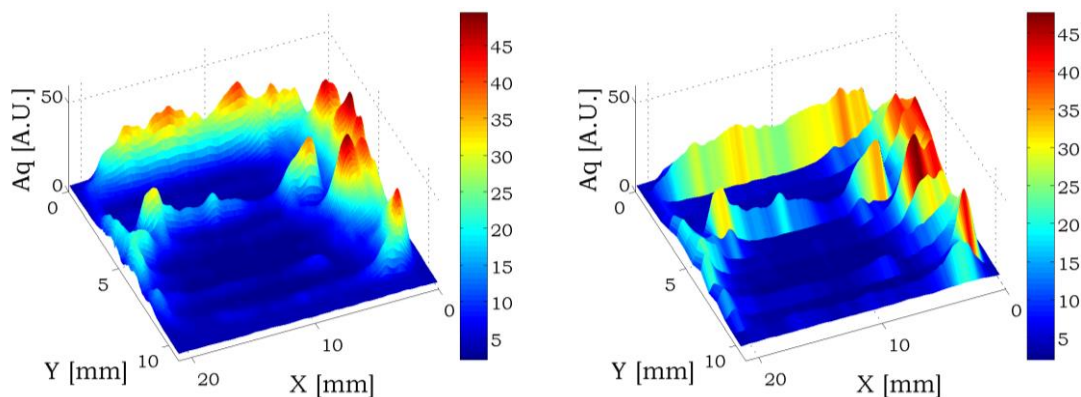
Figure 7; high resolution (left) and low resolution (right) 3D representation of measured Aq covering one whole polished surface after 32 polishing passes (8 nm Sa).
