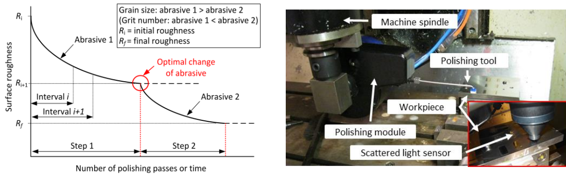
Figure 2; Schematic of surface generation in sequential RAP process depicting the optimal time for change of the abrasive media (left) and experimental setup (right).
