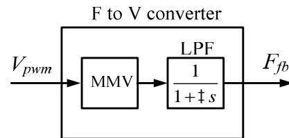
Fig. 8. Frequency to voltage (F to V) converter.
