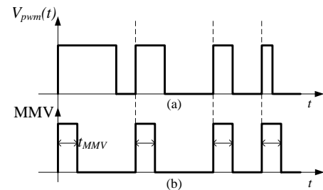
Fig. 7. Operation of the MMV a) the PWM output signal of the comparator, b) the output signal of the mono-stable multi-vibrator.
