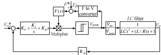
Fig. 6. The proposed fixed frequency self-oscillating control system.
