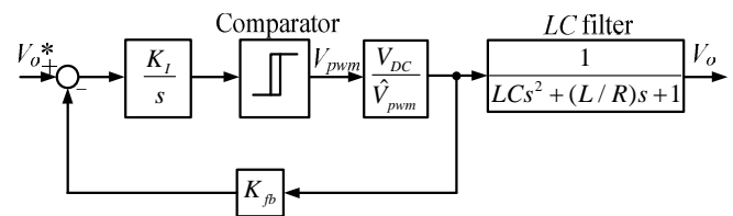
Fig. 1. A basic voltage-mode hysteresis controller.
