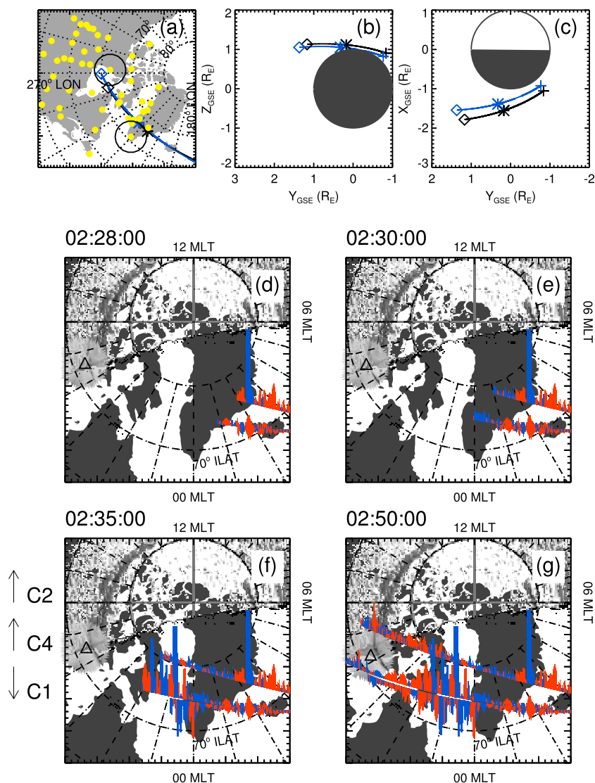
Figure 3. Figure showing the locations of Cluster 1 (black), Cluster 4 (blue), and the ground-based instrumentation used in this study. (a) The spacecraft foot points in geographic latitude and longitude. The crosses and diamonds show the spacecraft locations at 02:30 and 02:45 UT, respectively. The underlying map shows the locations of the ground magnetometer stations (yellow dots) and the fields of view of the RANK and NRSQ all-sky imagers at 02:30 UT. (b and c) The locations of Cluster 1 and Cluster 4 projected on the YZ and YX GSE planes, respectively. (d–g) The spacecraft foot point tracks from Cluster 1, Cluster 2, and Cluster 4 up to 02:28, 02:30, 02:35, and 02:50 UT. Overlaid on the spacecraft track are the magnetic field gradients perpendicular to the spacecraft track and the Tsyganenko and Stern [1996] magnetic field (negative gradients in red, positive gradients in blue). Gradients from Cluster 1 point down the page, and gradients from Cluster 2 and Cluster 4 point up the page. The dayside auroral data are from a single image compiled from DMSP SSUSI data from around 02:40 UT. Also plotted are auroral data from the THEMIS ASI at RANK projected to 110 km altitude. Auroral data are plotted in gray scale with darker colors indicating brighter aurora. An animation incorporating Figures 3d–g is provided in the supporting information.
