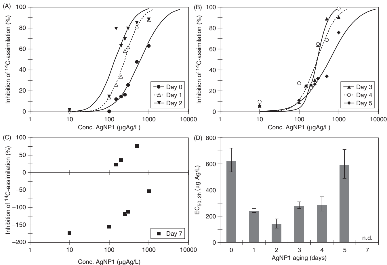
Figure 3. Concentration–response data and fitted curves by Log457 from 2-h algal ^{14}\text{C} -assimilation algal tests with AgNP1 after aging in ISO 8692 algal medium (A) for 0–2 days, (B) for 3–5 days, (C) for 7 days. The \text{EC}_{50} -values with 95% confidence intervals are plotted for suspensions aged for 0–7 days (D).
