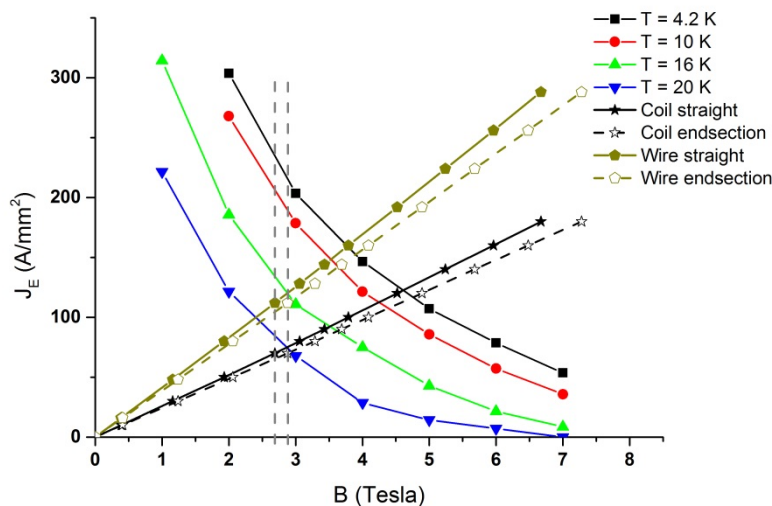
Figure 3. Load line of \text{MgB}_2 pole coil positioned in a 10 MW direct drive wind turbine generator. A coil J_{Ecoil} = 70 \text{ A/mm}^2 is desirable and corresponds to a J_{Ewire} = 112 \text{ A/mm}^2 taking insulation and spacers into account (crossing of vertical dashed line). The J_E of the wire includes the \text{MgB}_2 tape (3.0 mm x 0.5 mm) and a Cu strip for stabilization (3.0 mm x 0.2 mm) [7]. Operation at 2 T seems possible at 20 K whereas T = 10\text{-}15 \text{ K} is needed for 3 T operation.
