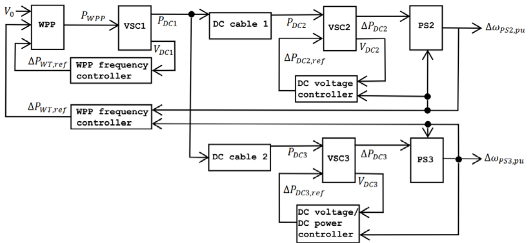
Figure 9. Overview of the block diagram of the VSC-HVDC intertie system and main controllers
