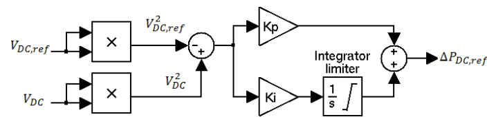
Figure 2. Centralized DC voltage control with fixed onshore DC voltage reference
