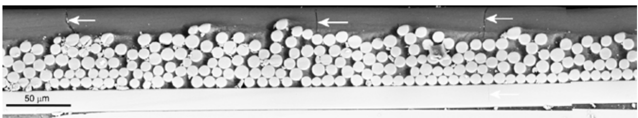
Fig. 1. Micrograph of polished edge showing cracks (indicated by arrows) and broken fibre.
