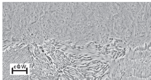
Fig. 3. SEM image of the Interface between the pearlitic (lower) and martensitic (upper) phases in a rail. The martensitic layers is produced when the surface of the rail is heated to more than 727 °C and rapidly cooled.
