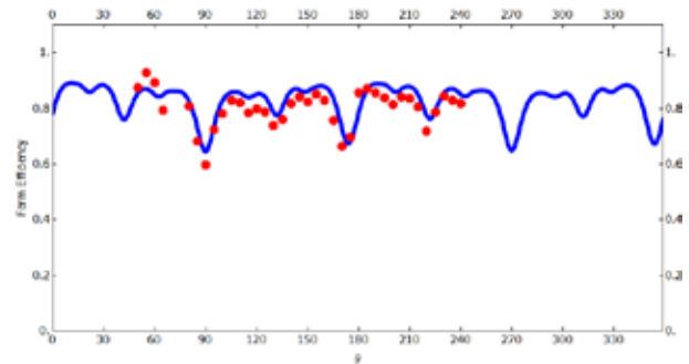
Fig. 2. Predicted (blue line) and observed farm efficiency for Horns Rev 1 as a function ten minutes average wind direction. The hub height wind speed is 9 \pm 1 m/s with neutral stability. The dips correspond to wind directions aligned with turbine rows. Measured data only covers directions where the met mast is outside the farm wake.
