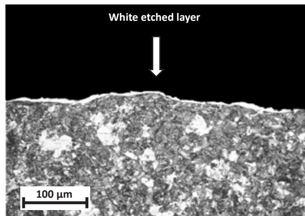
Fig. 2. Optical microscopy image. The pearlitic rail has a white etched layer at the surface which is marked by an arrow.
