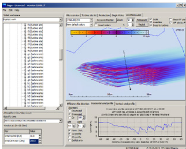
Fig. 1. Fuga as it appears on at computer screen.
