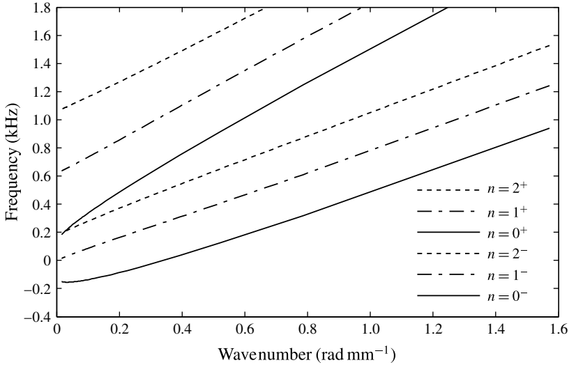
FIGURE 2. Dispersion relation for the two \pm branches of the three modes described by (2.20). Condition; \Omega = 2.0 \times 10^3 rad s ^{-1} , W = 6.3 m s ^{-1} and r_c = 2.3 mm.
