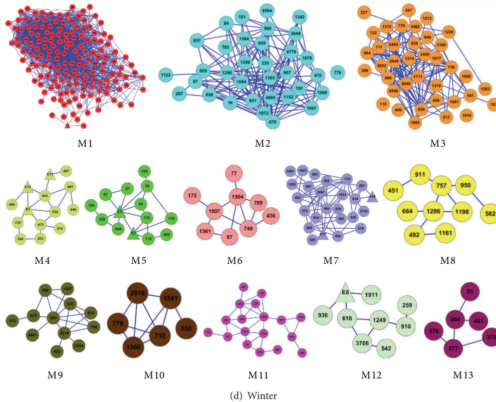
FIGURE 5: The structure of microbial interaction pattern detected by s -NMF algorithm in four seasonal networks. (○-OTU, △-environmental factor).
