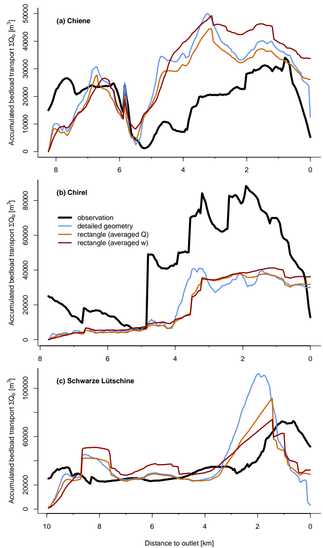
Figure 3. Comparison of the effects of different channel representations on accumulated bedload transport estimates simulated with the Tom Sed model in three Swiss mountain rivers. See Table 2, text, and Stephan (2012) for details.
