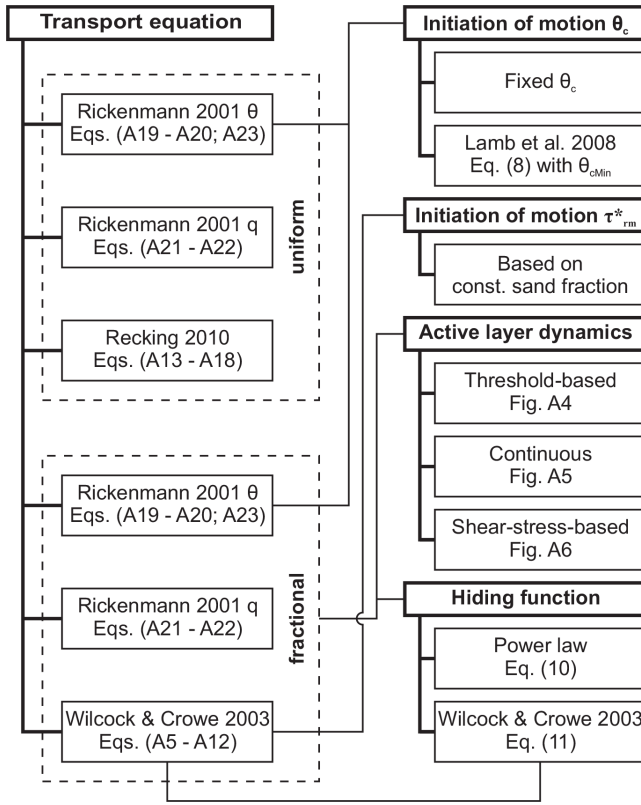
Figure A1. Simplified summary diagram of the bedload transport part of sedFlow, showing a selection of the most important general types of functions (bold type face) and their selectable realisations (regular type face). For the transport equations of Rickenmann (2001), versions for both fractional and uniform grain sizes are implemented in sedFlow. Among the implemented equations, only the \theta -based ones of Rickenmann (2001) use \theta_c to determine the initiation of bedload motion. The selection of a hiding function and active surface layer dynamics is only necessary if a fractional transport equation is used. The transport equation of Wilcock and Crowe (2003) is always combined with their proposed hiding function and uses \tau_{rm}^* to determine the initiation of bedload motion.
