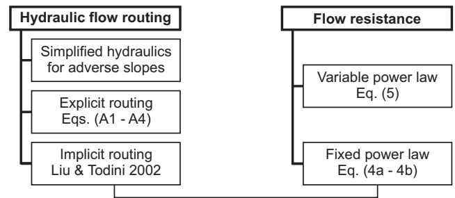
Figure A2. Simplified summary diagram of the hydraulic part of sedFlow, showing a selection of the most important general types of functions (bold type face) and their selectable realisations (regular type face). The implicit flow routing of Liu and Todini (2002) is always combined with a fixed power law flow resistance.
