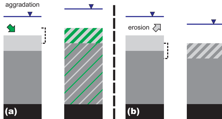
Figure A5. Qualitative sketch of continuous interaction between the active surface layer and subsurface alluvium. The water level is displayed in blue, the active surface layer with its constant thickness is light grey, the subsurface alluvium consisting of one layer with variable thickness is dark grey and bedrock is black. The dashed bracket indicates the position of the active surface layer after aggradation or erosion. In case of aggradation (a) , the material input from upstream, which is displayed in green, is added to the active surface layer, which is instantaneously homogenised. Any material of the homogenised active surface layer, which exceeds the constant thickness, is transferred to the subsurface alluvium, which is instantaneously homogenised as well. Any homogenisation process is displayed by diagonal stripes. In case of erosion (b) , the sediment deficit of the active surface layer is replaced by material from the subsurface alluvium and the active surface layer is instantaneously homogenised.
