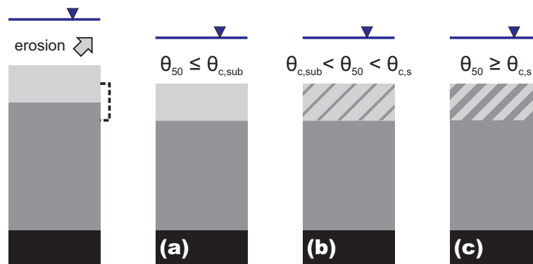
Figure A6. Qualitative sketch of shear-stress-based interaction between the active surface layer and subsurface alluvium. For an explanation of the symbols see the caption of Fig. A5. In this approach, the aggradation case is treated identically to the continuous update approach displayed in Fig. A5a. For erosion, three cases are differentiated, with the representative dimensionless shear stress \theta_{50} increasing from case (a) to case (c) . If \theta_{50} equals or exceeds the threshold for the active surface layer \theta_{c,s} (c) , the layers interact in the same way as in the continuous update approach displayed in Fig. A5b. If \theta_{50} does not exceed the threshold for the subsurface alluvium \theta_{c,sub} (a) , the volume deficit of the active surface layer is replaced by material from the subsurface alluvium, but the grain-size distribution of the active surface layer remains constant. For the intermediate case with \theta_{50} greater than \theta_{c,sub} and smaller than \theta_{c,s} (b) , the influence of the grain-size distribution of the subsurface alluvium on the grain-size distribution of the active surface layer is interpolated linearly between cases (a) and (c) .
