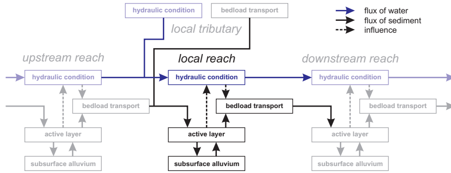
Figure 1. Simplified overview over the main process interactions within the sedFlow model.
