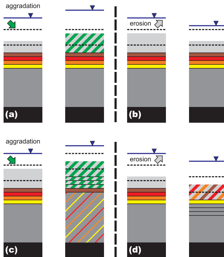
Figure A4. Qualitative sketch of threshold-based interaction between the active surface layer and subsurface alluvium. The water level is displayed in blue, the active surface layer with its variable thickness is light grey and bedrock is black. The subsurface alluvium consists of several strata layers with user-defined constant thickness displayed in reddish colours and one base layer with variable thickness displayed in dark grey. The horizontal dashed lines indicate the thresholds for the thickness of the active surface layer. In case of aggradation ( a and c ), the material input from upstream, which is displayed in green, is added to the active surface layer, which is instantaneously homogenised. Any homogenisation process is displayed by diagonal stripes. If the thickness of the active surface layer does not exceed its thresholds after aggradation or erosion ( a and b ), the thresholds of the active surface layer and the layers of the subsurface alluvium remain constant. If the active surface layer thickness exceeds its upper threshold after aggradation ( c ), the complete system of layers and thresholds is shifted upwards so that the upper boundary of the active surface layer is in the middle between its thresholds. The upper strata layers are populated with material from the homogenised active surface layer, while the material of the lower strata layers is added to the base layer, which is instantaneously homogenised. If the active surface layer thickness exceeds its lower threshold after erosion ( d ), the complete system of layers and thresholds is shifted downwards so that the upper boundary of the active surface layer is in the middle between its thresholds. The lower strata layers are populated with material from the base layer, while the material of the upper strata layers is added to the active surface layer, which is instantaneously homogenised.
