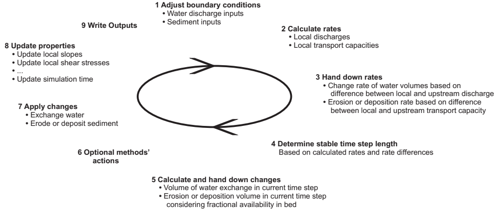
Figure A3. Simplified summary diagram of a time step in sedFlow. The timing of the optional methods' actions has been selected in a way that all changes, such as, e.g., erosion or deposition volumes, are readily calculated and available for possible modifications before the changes, such as, e.g., erosion or deposition, are then actually applied.
