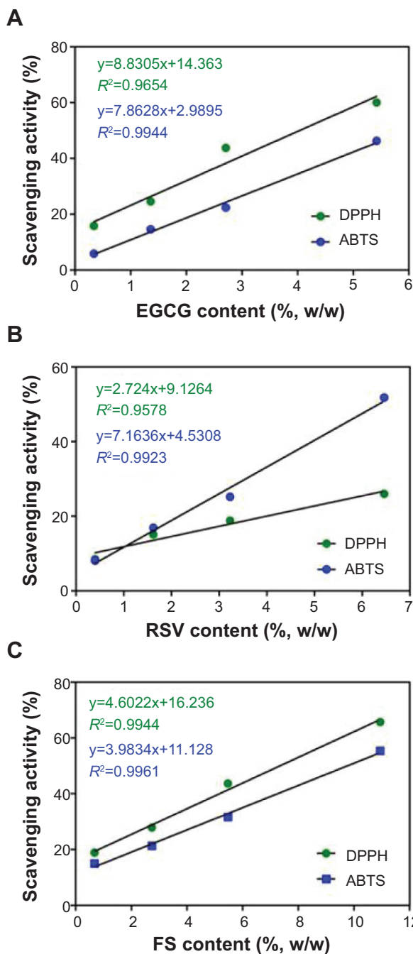
Figure S5 Correlation between radical-scavenging capacity assays (DPPH and ABTS) of EGCG-GNPs, RSV-GNPs, and FS-GNPs and (A) EGCG, (B) RSV, and (C) FS content (% w/w).
