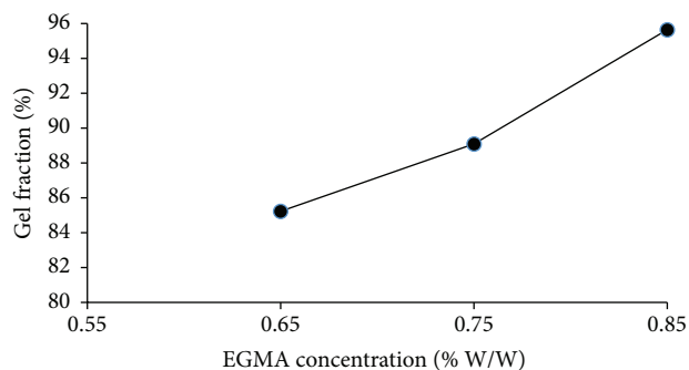
FIGURE 11: Effect of cross-linking agent concentration (EGDMA) on gel fraction of AA/Gelatin hydrogels.
