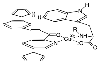
Figure 1. Transition-state assembly suggested 15 for the aqueous Lewis-acid-catalyzed Diels–Alder reaction of 1 with 2 .
