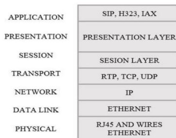
Figure 1. VoIP reference model.
