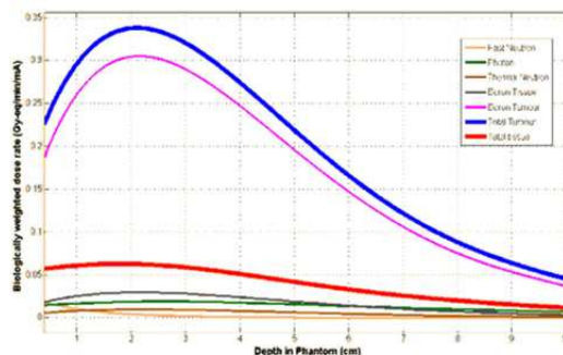
Figure 1: Comparison between the dose delivered to tumour and healthy cells using BNCT for realistic uptakes on the carrier compound BPA.
