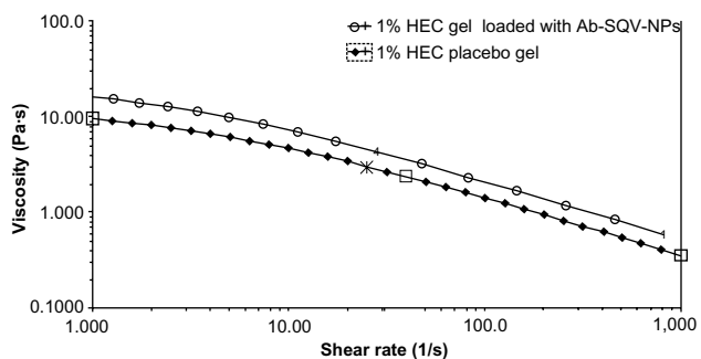
Figure 4 Steady-state flow curves of 1% hydroxyethylcellulose (HEC) placebo gel (filled diamonds), and 1% HEC gel containing antibody-conjugated saquinavir-loaded nanoparticles (Ab-SQV-NPs; 5 mg NPs/g gel, empty circles) at a measurement temperature of 37°C. Viscosity profiles were performed as a single measurement.
