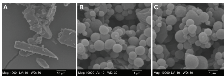
Figure 2 Representative scanning electron micrographs of (A) raw unprocessed cyclosporine A and cospray-dried cyclosporine A: dipalmitoylphosphatidylcholine/ dipalmitoylphosphatidylglycerol ratio of (B) 25:75 (1:3) and (C) 75:25 (3:1).
