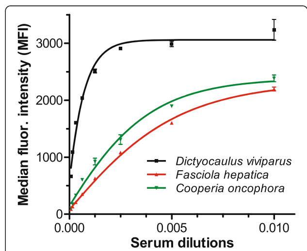
Fig. 2 Results for the triplex assay using serum dilutions of cattle infected with Dictyocaulus , Fasciola and Cooperia . Five parameter logistic regression curves were calculated based on median fluorescence intensity (MFI) values. Beads are coupled with recombinant antigen for the detection of Cooperia oncophora (green), Dictyocaulus viviparus (black) and Fasciola hepatica (red). Artificial mixtures of sera from animals infected with the target species was used. Dilutions are presented as 0.005 ± 1:200
