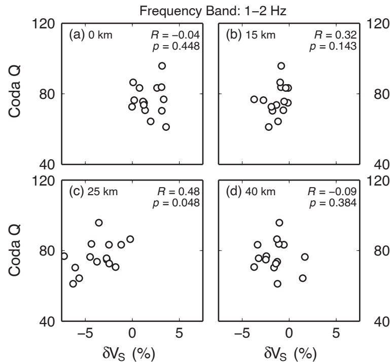
Figure 4 Relation between \delta V_S and coda Q at the 1- to 2-Hz frequency band. Plot of \delta V_S (Matsubara et al. 2008) at (a) 0-, (b) 15-, (c) 25-, and (d) 40-km depths versus coda Q at the 1- to 2-Hz frequency band. R shows the correlation coefficient; p is the p value.
