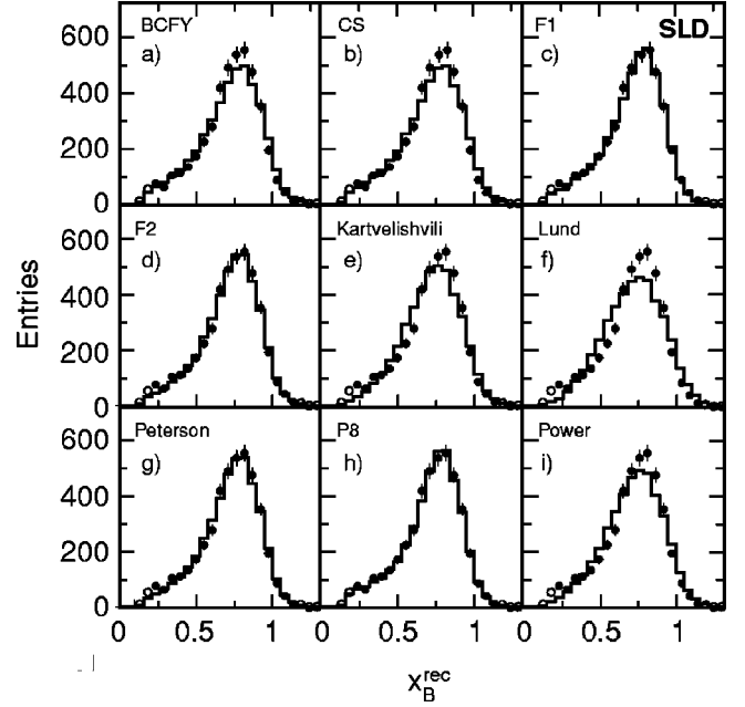
FIG. 9. The background-subtracted distribution of reconstructed B -hadron energy (points). Also shown (histograms) are the predictions of the optimized functional forms. Data points excluded from the fit are represented by open circles.
