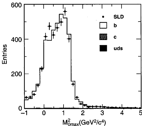
FIG. 4. Distribution of the reconstructed M_{0max}^2 for the final selected sample (see text). The simulated distribution is also shown (histogram) in which the flavor composition is indicated: b (open), c (cross hatched), and uds (dark shaded).
