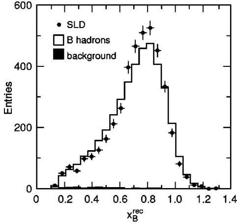
FIG. 7. Distribution of the reconstructed scaled B -hadron energy (points) and the default Monte Carlo simulation (histogram). The solid histogram shows the simulated non- B background.
