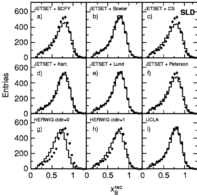
FIG. 8. The background-subtracted distribution of reconstructed B -hadron energy (points). Also shown (histograms) in (a)–(f) are the predictions of the optimized models within JETSET (see text). (g) and (h) show the predictions of HERWIG, and (i) of the UCLA model. Data points excluded from the fit are represented by open circles.
