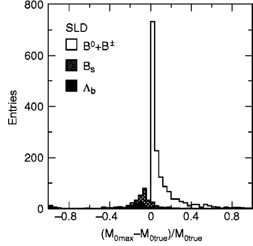
FIG. 2. The relative deviation of the maximum missing mass from the true missing mass for simulated B hadron decays; the contributions from different B species are indicated separately: B^0 and B^\pm (open), B_s^0 (cross-hatched), and \Lambda_b (dark shaded).
