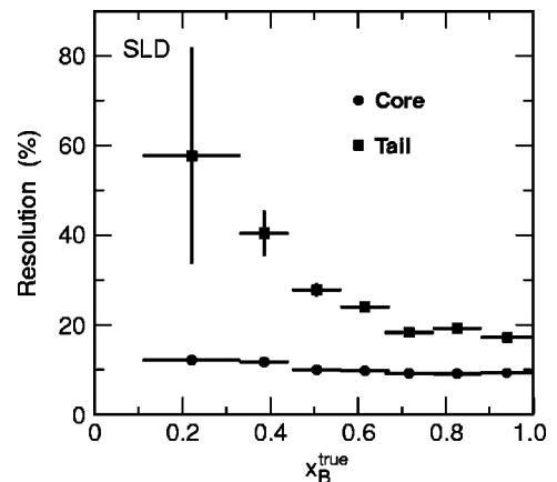
FIG. 6. The fitted core and tail widths (see text) of the B -energy resolution as a function of the true scaled B -hadron energy.
