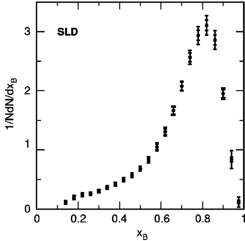
FIG. 11. Final distribution of the weakly decaying scaled B -hadron energy. In each bin the central value is the average of the eight distributions shown in Fig. 10, the inner error bar represents the experimental error, and the outer error bar represents the sum in quadrature of the experimental and unfolding errors.
