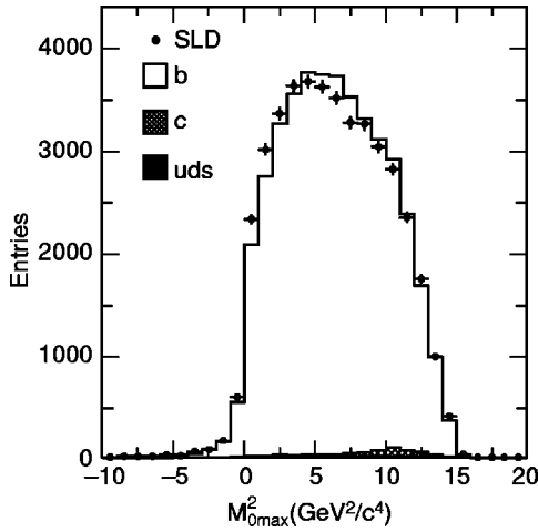
FIG. 3. Distribution of the reconstructed M_{0max}^2 for the selected vertices (points). The simulated distribution is also shown (histogram) in which the flavor composition is indicated: b (open), c (cross hatched), and uds (dark shaded).
