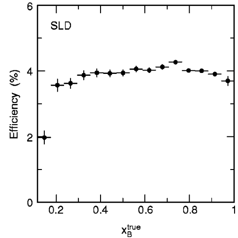
FIG. 5. The simulated efficiency for selecting B hadrons as a function of the true scaled B -hadron energy, x_B^{true} .
