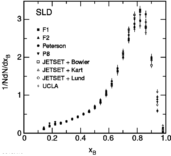
FIG. 10. Distributions of the scaled weakly decaying B -hadron energy unfolded using different input models or functions (see text).
