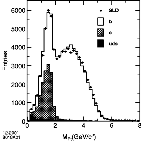
FIG. 1. Distribution of the reconstructed P_t -corrected vertex mass (points). The simulated distribution is also shown (histogram) in which the flavor composition is indicated: b (open), c (cross hatched), and uds (dark shaded).
