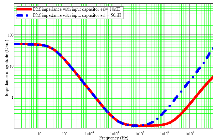
Fig. 18. The comparison between two DM impedances profile about two values of the " esl = \{10nH, 50nH\} " of the input capacitors C_f .
