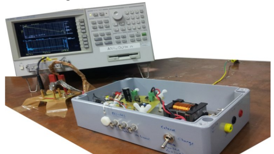
Fig. 10. The identification of converters' parameters.
