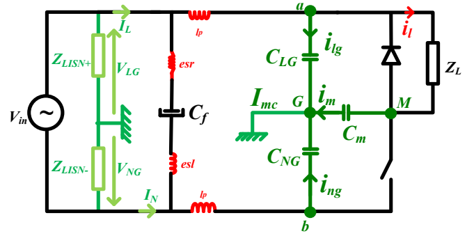
Fig. 8. The buck converter under study.
