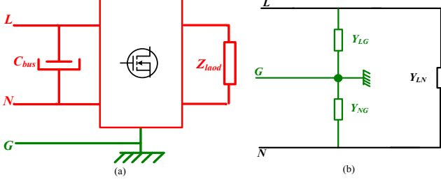
Fig. 2. Converter circuit topology: (a) converter circuit designed as an active multi-port circuit, (b) The equivalent \pi -quadrupole circuit
