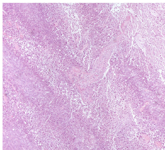
Figure 9 DDMC-p53 complex plus cisplatin.
