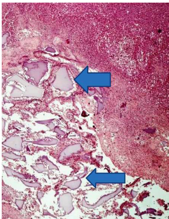
Figure 6 DDMC with p53.
