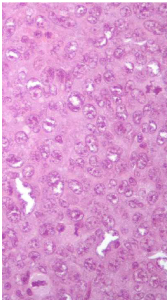
Figure 11 Microwave group. Note: Magnification 100×.
