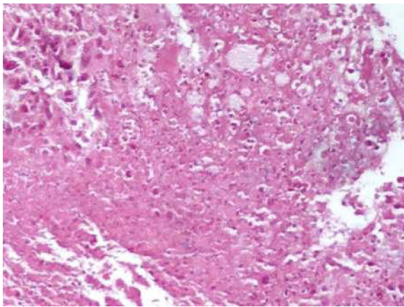
Figure 10 Cisplatin group. Note: Magnification 100×.
