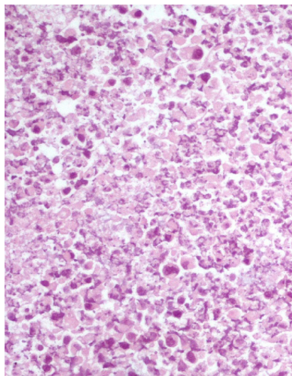
Figure 8 DDMC with p53 plus microwave group.
