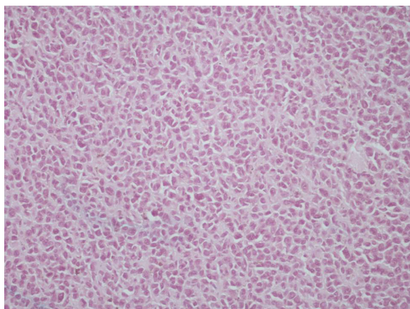
Figure 7 Control group (without therapy).
