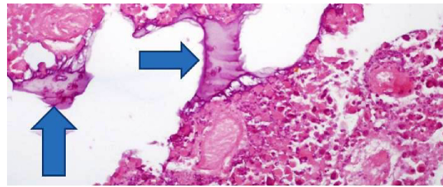
Figure 12 DDMC-p53 plus cisplatin plus microwave group. Notes: Magnification 100×. The blue arrows indicate the DDMC-p53 complex within the tissue. Abbreviation: DDMC, 2-diethylaminoethyl-dextran methyl methacrylate copolymer.
