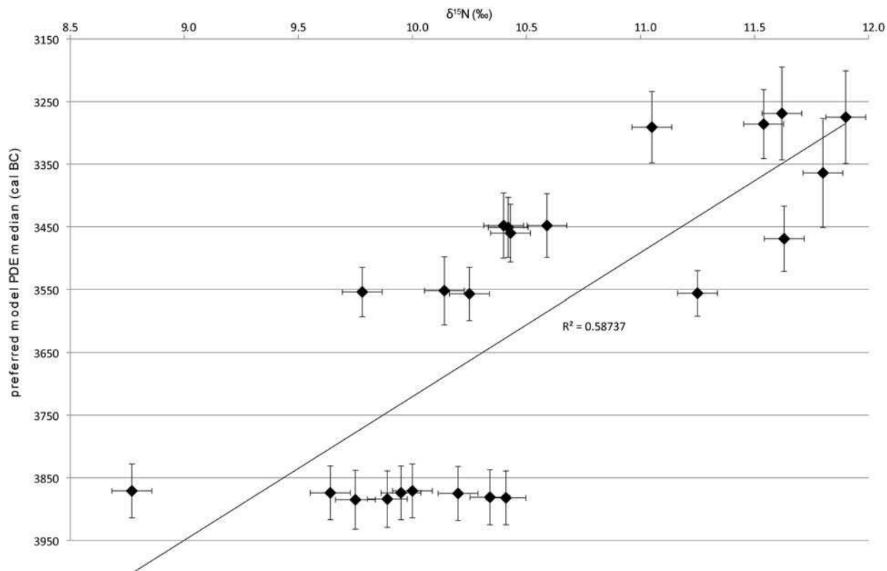
Fig. 12. Changes in \delta^{15}\text{N} values over time. The horizontal axis plots \delta^{15}\text{N} (with estimated analytical error); the vertical axis plots the posterior density estimate median and standard deviation range from the preferred model (model 2, Fig. 8)
