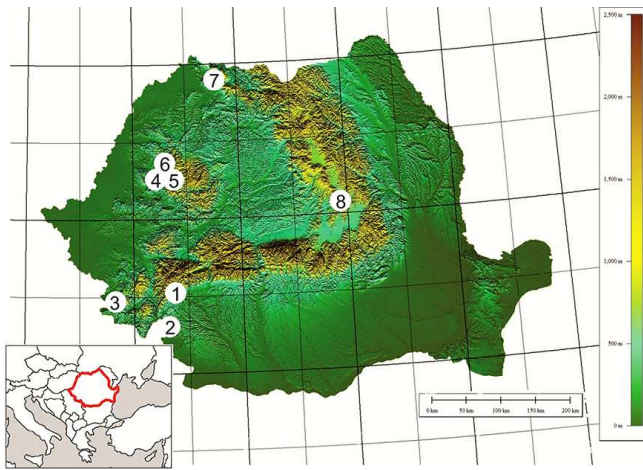
Figure 1. Location of Romanian palaeoclimate records and meteorological stations mentioned in the text: 1 – Ascunsă Cave; 2 – Drobeta meteorological station; 3 – Poleva Cave; 4 – Urşilor Cave; 5 – V11 Cave; 6 – Stâna de Vale meteorological station; 7 – Steregoiu peat bog; 8 – Sfânta Ana Lake.
