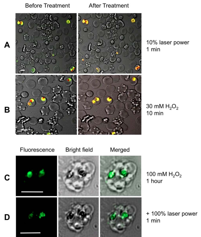
Figure 5. The parasite DV remains intact in parasites subjected to oxidative stress. (A) and (B) are confocal micrographs showing the redistribution of acridine orange fluorescence in intact parasitized erythrocytes subjected either to (A) 1 min illumination with the microscope's laser, or (B) 10 min exposure to 30 mM H_2O_2 . Prior to the treatment the DV fluoresces red and the parasite cytosol fluoresces green. Both treatments resulted in a loss of red fluorescence from the region of the DV. (C) and (D) show the retention of fluorescein-dextran within the DV of mature, isolated D10 trophozoites (there are two visible in the image) following exposure to 100 mM H_2O_2 for 1 hour (C), followed by excitation with a 488 nm laser line at full power for 1 min (D). Neither the high concentration of H_2O_2 alone, nor the subsequent additional intense light exposure resulted in any redistribution of the fluorescein-dextran from the DV of the parasites (visible as dark regions, coinciding with the hemozoin crystals, in the bright-field images), from which it may be concluded that the DV remained intact. All scale bars (shown in white) are 5 \mu m. doi:10.1371/journal.pone.0058933.g005
