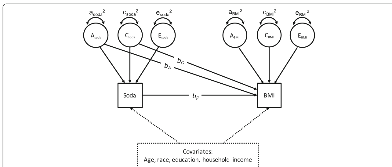
Fig. 2 Quasi-causal twin model, controlling for covariates. A additive genetic component; C shared environment component; E non-shared environment component; b_A and b_C amount of residual variance of body mass index attributable to the genetic and shared environment, respectively; b_P phenotypic association
