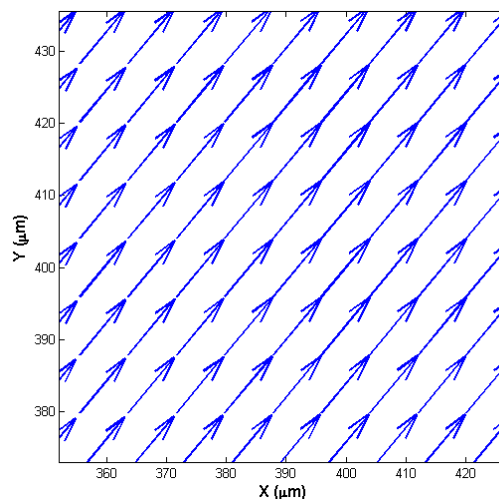
Figure 2.17. Fundamental shear S_{01} for the vector plot \vec{U}_t = \vec{U}_x + \vec{U}_y .
