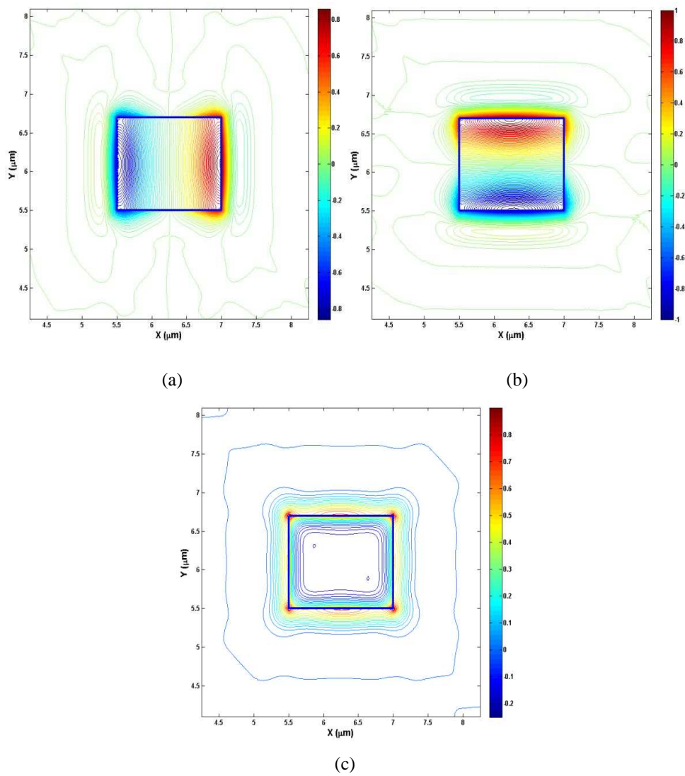
Figure 5.30. The displacement vector plots of (a) U_x (b) U_y and (c) U_z components of the R1 ( U_{12}^y ) mode at k = 10.0 \mu\text{m}^{-1} .
