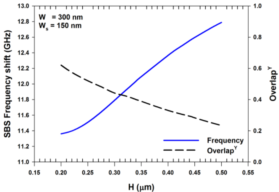
Figure 6.15. Variation of H with overlap Y and SBS frequency shift (GHz).
