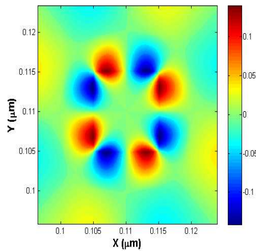
Figure 3.19. The U_z displacement fields profile of the torsional mode at k=200 \text{ m}^{-1} .
