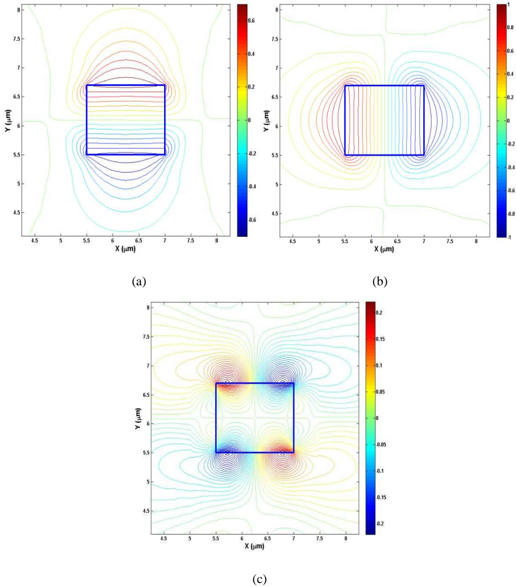
Figure 5.27. Displacement vector profiles (a) U_x (b) U_y , and (c) U_z of the T1 U^y_{21} mode at k=1.5 \mu\text{m}^{-1} .
