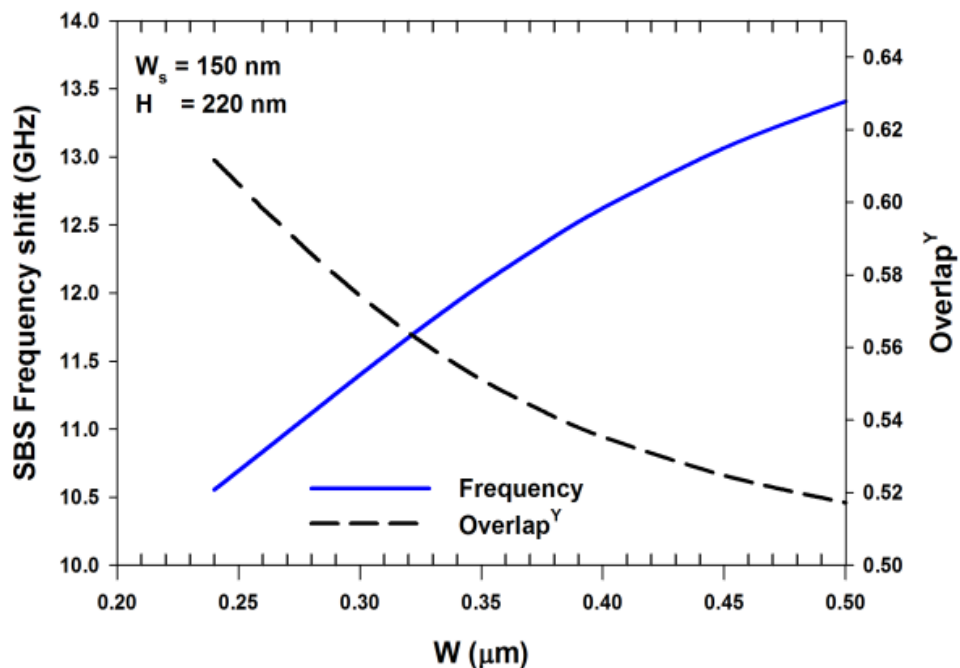
Figure 6.17. Variation of W with (a) \text{overlap}^y and SBS frequency shift (GHz).
