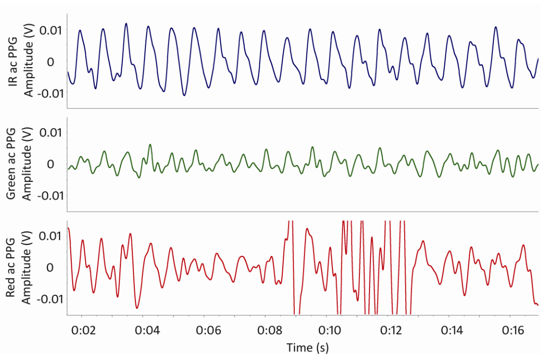
Figure 10.2: Typical red, green and infrared ac PPG signals from the LD flap prior to its transfer.
