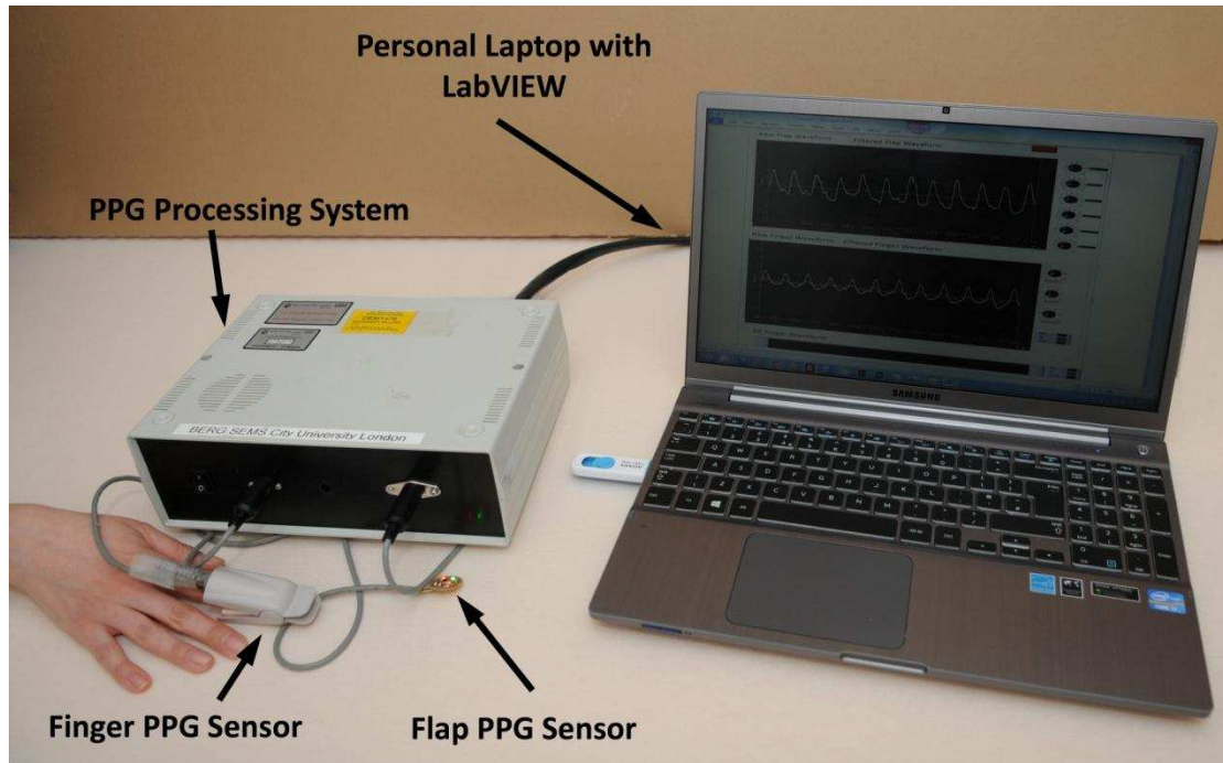
Figure 7.24: Photograph demonstrating the setup of the developed PPG processing system and sensor on a volunteer.
