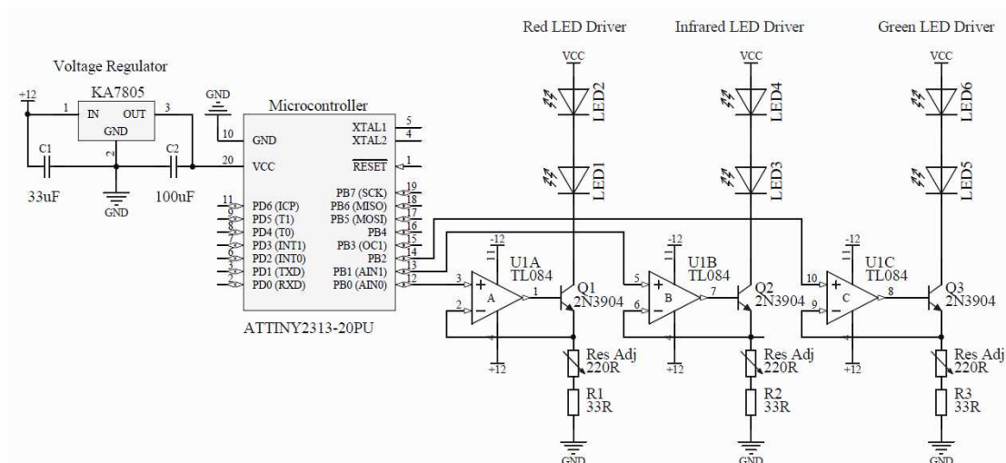
Figure 7.3: Schematic drawing of the LED current driver circuit.
