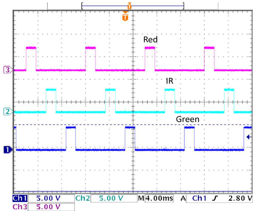
Figure 7.18: The timing signals used for driving the LEDs and demultiplexing the output of the transimpedance amplifier as observed on an oscilloscope.
