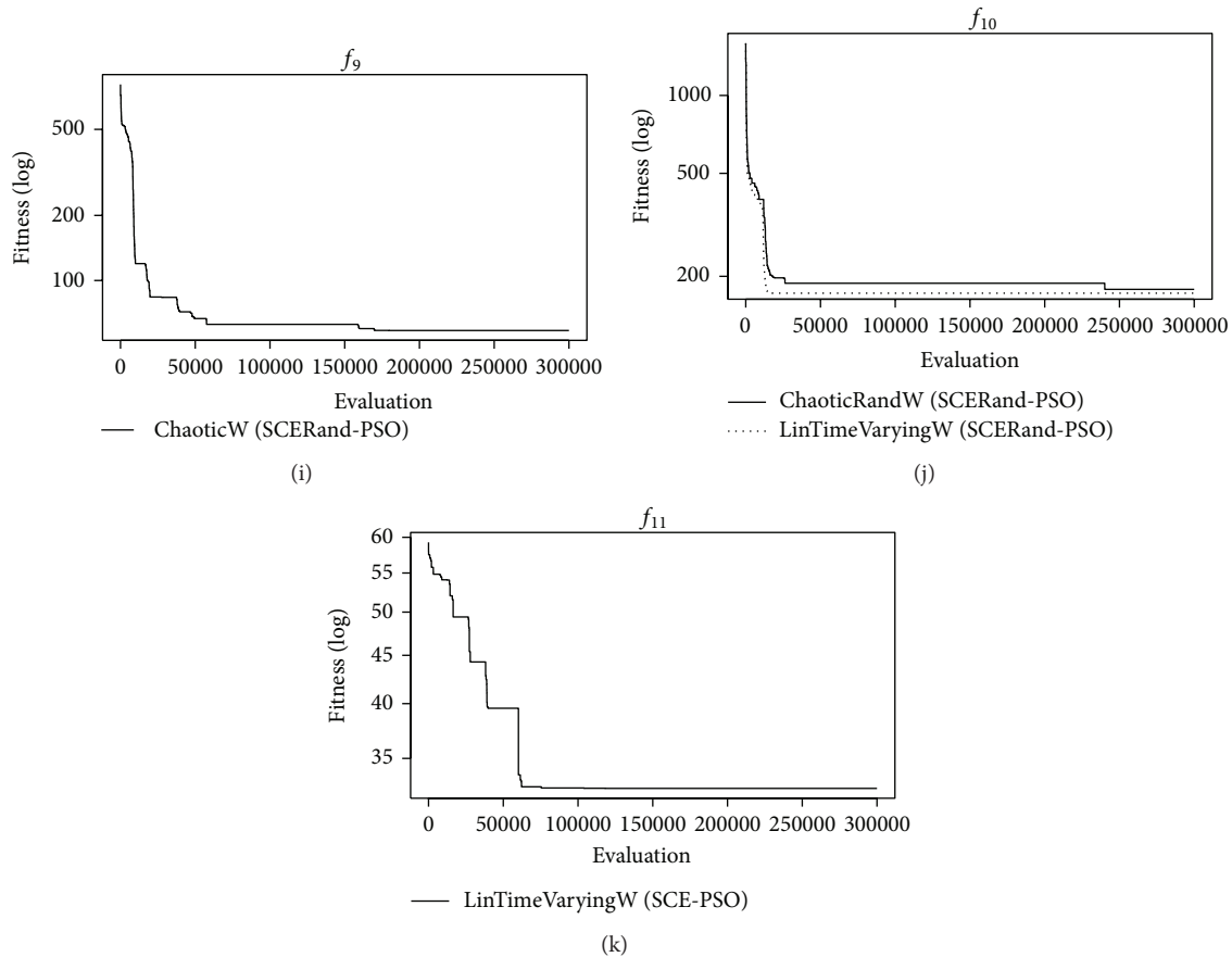
FIGURE 1: Convergence graphs for best fitness of the best modifications and strategy of PSO for functions f_1 - f_{11} according to Table 3.
