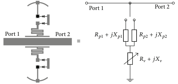
FIGURE 3: Equivalent circuit of the band-notched structure.
